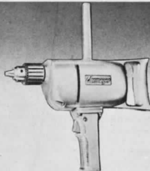
No. 510 — ½" DRILL WITH FAMOUS GEARED CHUCK. Multiple ball thrust bearing and self-lubricating bearings. Capacity in steel, ½"; in hard wood, 1". No load speed, 500 RPM. 115 V. AC-DC. Switch with automatic shut-off and lock. 12¾" long. LIST $39.95.
