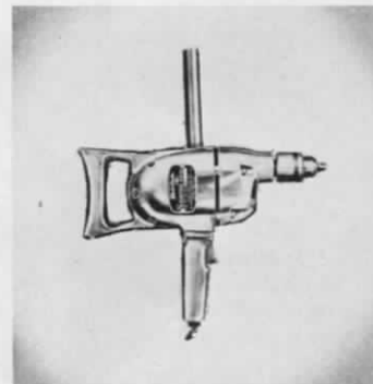
No. U-20 — BLACK & DECKER 1/2" UTILITY DRILL. Drills from 1/8" to 1/2" in steel, drives wood augers up to 1" and Hole Saws up to 3". 115 volts. A.C. or A.D. 375 RPM. Instant-Release Trigger Switch. With Hex-Key Chuck. LIST $53.50.
