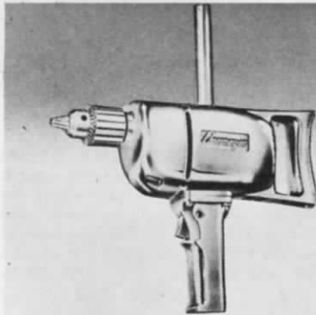
No. 520 — ½" DRILL WITH FAMOUS GEARED CHUCK. Streamlined design for operator comfort and close quarter use. ½" steel capacity, 1" hard wood. No load speed, 500 RPM. 115 voltage. AC-DC. Switch with automatic shut-off and lock. Silver finish. 12¾" long. LIST $49.95.
