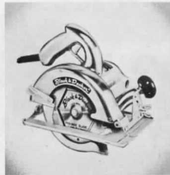
No. 73 — BLACK & DECKER HEAVY-DUTY SAW. With 7 1/4" Blade—2 3/8" depth of cut. Heat-treated heavy-duty gears and lubricant-sealed ball bearings assures top performance. 4700 RPM no-load speed. 115 volt. A.C. or A.D. Instant-release switch. LIST $89.50.
