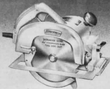
No. 700—DORMEYER PORTABLE POWER SAW. Positive fingertip adjustment for depth of cut ¼" to 2-3/16" at 45° bevel. Exclusive eye shield. No load speed, 5500 RPM. 115 voltage. AC-DC. Satin silver finish. 16 lb. ship. wt. LIST $49.95.
